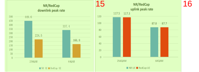
Figure 9: 2.1G Actual peak rate 17
