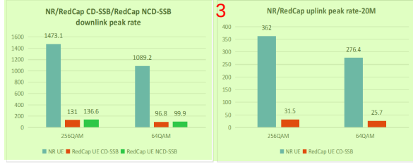
Figure 8: 3.5G Actual peak rate 5
