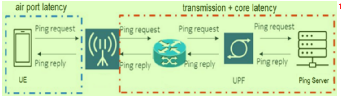
Figure 2: User-plane end-to-end latency composition
