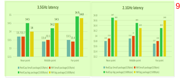
Figure 11: Actual user-plane end-to-end latency 10
