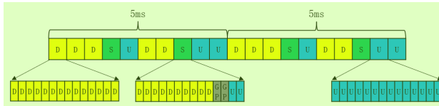
Figure 4: Frame Structure
